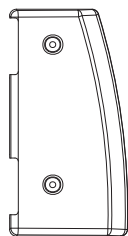
26. Thigh Pad Cover, L QTY 1
