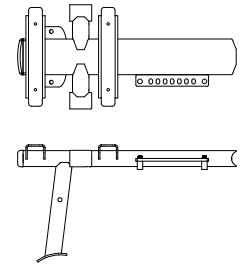
2. Seat Frame QTY 1
