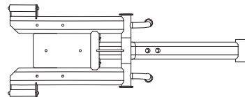
9. Swivel Frame QTY 1
