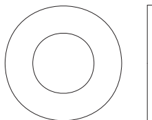
4. Washer, OD20 x ID10.5 x 1T QTY 12
