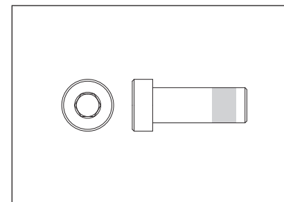
4. Bolt, 3/8-16 x 1" (25mm) socket head W/NP (black) QTY 3
