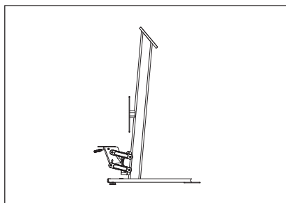
1. Front upright QTY 1
