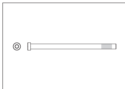
9. Bolt, 3/8-16 x 6-1/4" (159mm) socket head W/NP QTY 2
