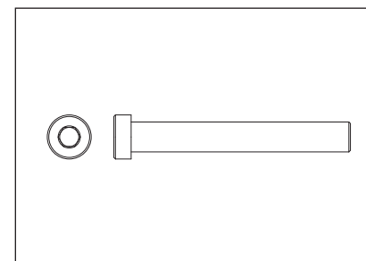
8. Bolt, 3/8-16 x 2-3/4" (70mm) socket head QTY 2
