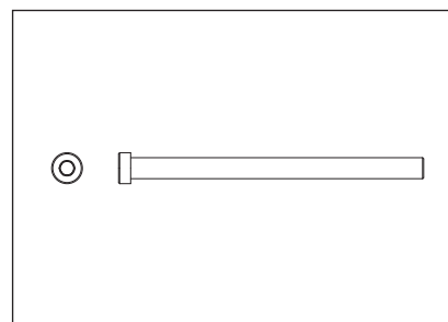
19. Bolt, 3/8-16 x 5-1/4" (133mm) socket head QTY 2
