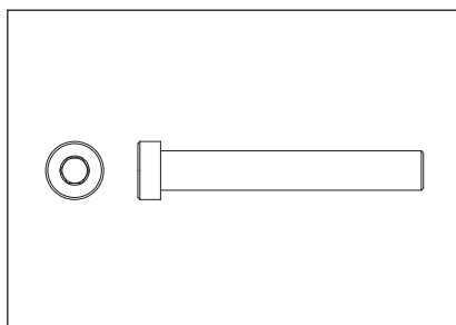
5. Bolt, 3/8-16 x 2-1/2" (64mm) socket head QTY 1
