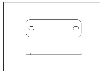
11. Plate, 50 x 155 x 4mm QTY 1
