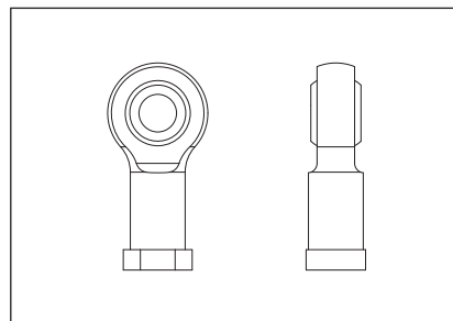
46. Rod end, M-12 female QTY 2
