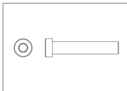
38. Bolt, 3/8-16 x 2" (51mm) socket head QTY 1
