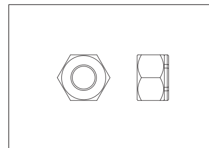
8. Nut, 3/8-16 x 11t LK ST ZN QTY 12
