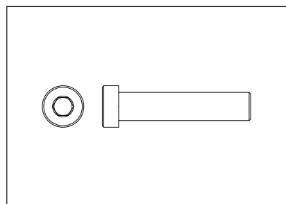
34. Bolt, 3/8-16 x 1-3/4" (45mm) socket head QTY 2
