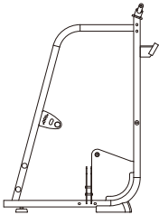
2. LPD Main Frame QTY 1
