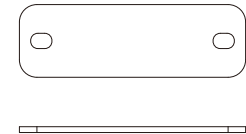
11. Plate, 50 x 155 x 4 mm QTY 1
