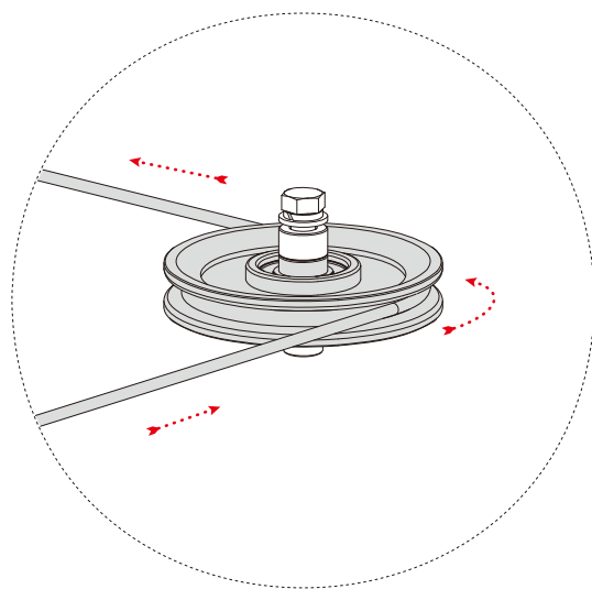
CABLE ROUTING
